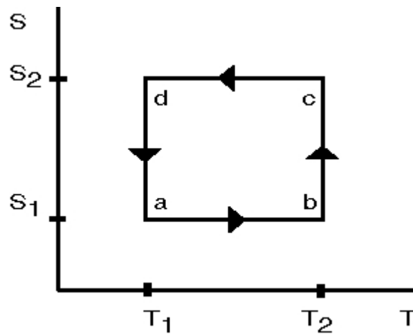
Figure 12.2: Temperature Cycle
