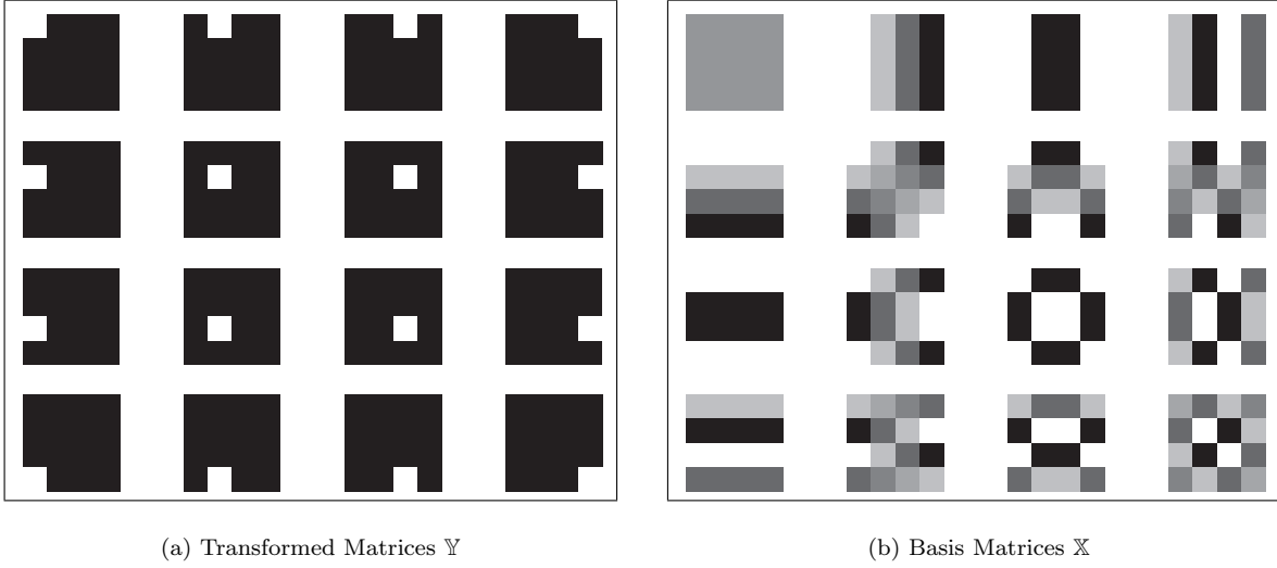
Figure 3.7: (a) 4 \times 4 pixel images representing the coefficients appearing in the matrix \mathbb{Y} from equation 3.15. And, (b) corresponding Inverse Discrete Cosine Transformations, these ICDTs can be interpreted as the base images that correspond to the coefficients of \mathbb{Y} .
