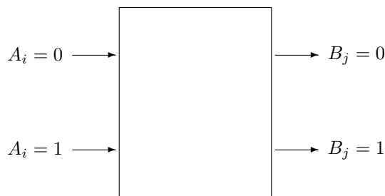
Figure 6.3: Binary Channel
